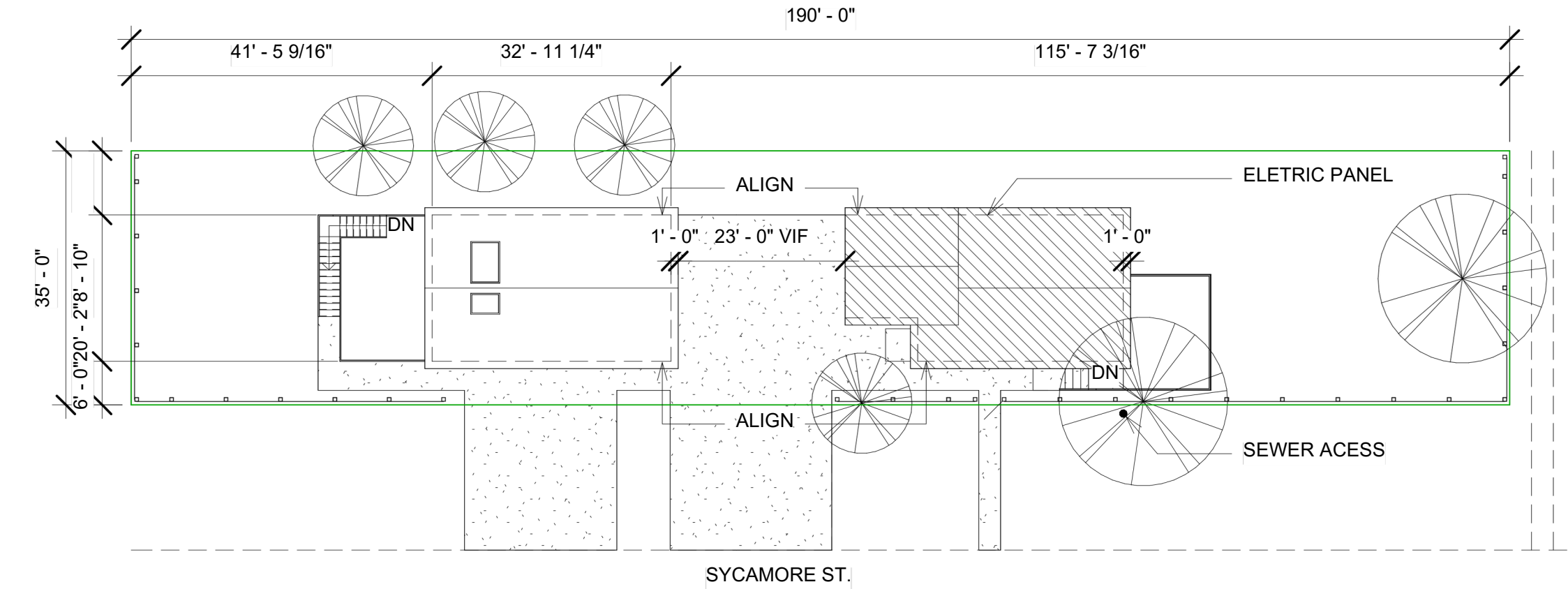
1 Proposed Site Plan 1" = 20'-0"
