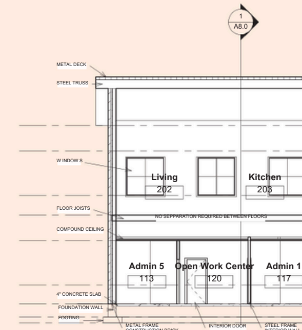
2 Transverse Section 1/8" = 1'-0"
