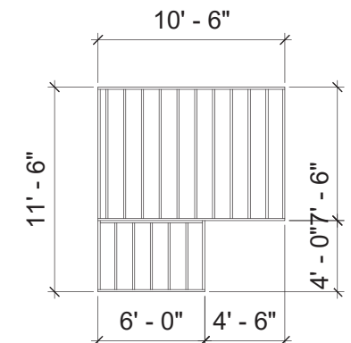
④ Detail Drawing 1/4" = 1'-0"
