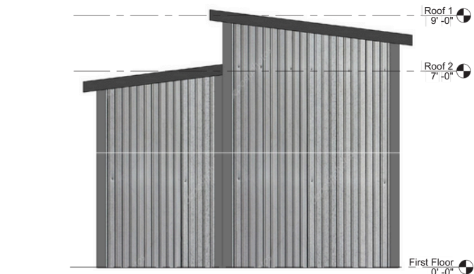
⑤ North Elevation 1/2" = 1'-0"
